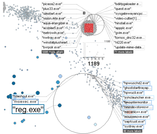
Figure 4: The size of the lens automatically changes according to data density.
