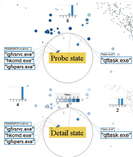
Figure 2: The "probe state" above shows only labels and summary statistics. The "detail state" below provides additional details and interactive filtering.
