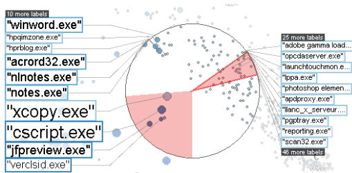
Figure 3: The pie segments over the lens allow users to scroll the list of labels.
