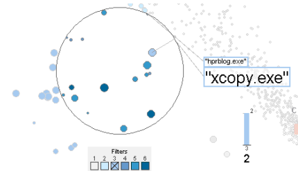
Figure 5: Label filtering: only the labels of applications used in 3 departments are shown.
