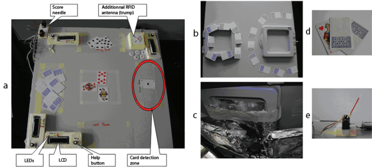
Figure 1: a) Overview of Tjass game board; b) Antenna positions and field jumping; c) Field reduction using Faraday cage; d) Tagged cards; e) The score needles.
